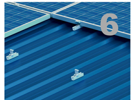
Fix the module on the mini rail by mid clamps and end clamps.
