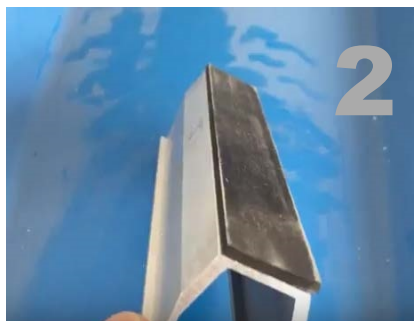
Each mini rail has been preassembled with one EPDM rubber pad.
